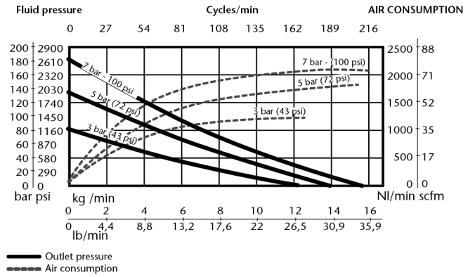
NLGI-0, 21 °C (70 °F) CAPACITY CURVE
