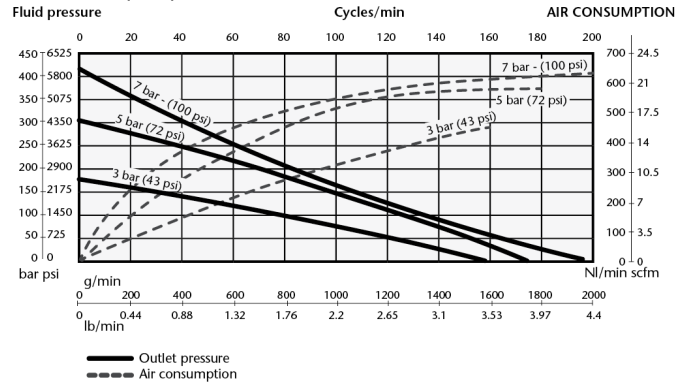
NLGI-2, 21 °C (70 °F) CAPACITY CURVE
